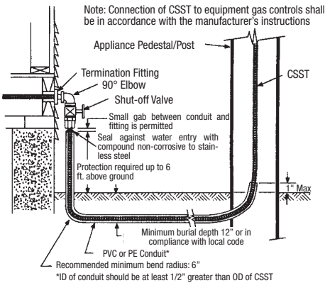
Figure 4.22 Fixed Outdoor Appliance (Underground Routing)
