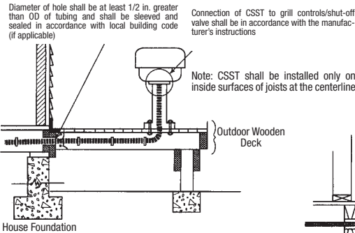
Figure 4.21 Fixed Outdoor Appliance (Deck Mounted)
