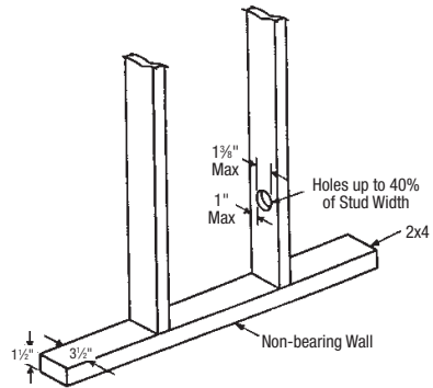
Figure 4.5 Holes in Bearing Walls
