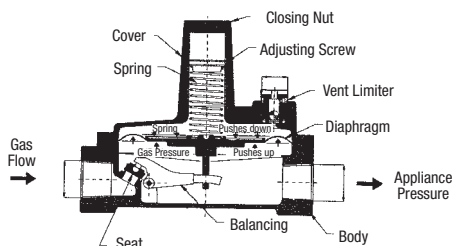
Figure 4.26 Pressure Regulator Diagram
