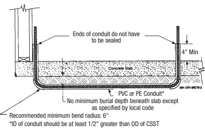
Figure 4.8 Installation in Non-Metallic Conduit Under Slab
