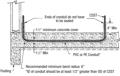
Figure 4.9 Installation in Non-Metallic Conduit In Slab
